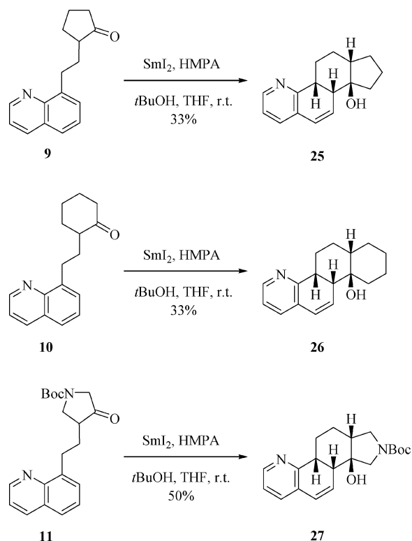
Scheme 8. Samarium diiodide promoted synthesis of azasteroid derivatives 25 and 26 and that of diazasteroid 27 .
